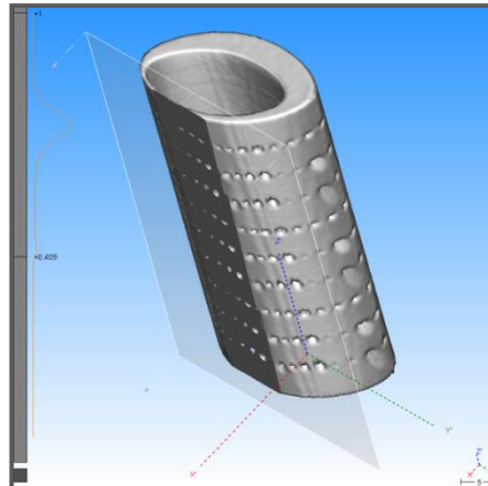
Hole locations at defined cross-section of CT scan data
