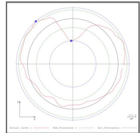
Roundness inspection & measurement of hole at defined cross section of CT
